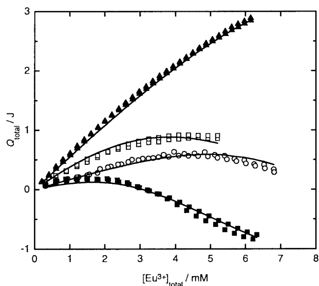
Fig. 4 Experimental and calculated (—) total heats observed for the titration of \text{pmdp} solutions with 0.102 \text{ M Eu}(\text{ClO}_4)_3\text{-}0.104 \text{ M HClO}_4\text{-}1.90 \text{ M NaClO}_4 . The calorimeter initially held 50 \text{ ml} of (▲) 0.0295 \text{ M pmdp-}1.96 \text{ M NaClO}_4 at \text{p[H]} 1.008 , (■) 0.00799 \text{ M pmdp-}1.98 \text{ M NaClO}_4 at \text{p[H]} 1.988 , (○) 0.0197 \text{ M pmdp-}1.96 \text{ M NaClO}_4 at \text{p[H]} 1.994 or (□) 0.0119 \text{ M pmdp-}1.87 \text{ M NaClO}_4 at \text{p[H]} 1.007 .
