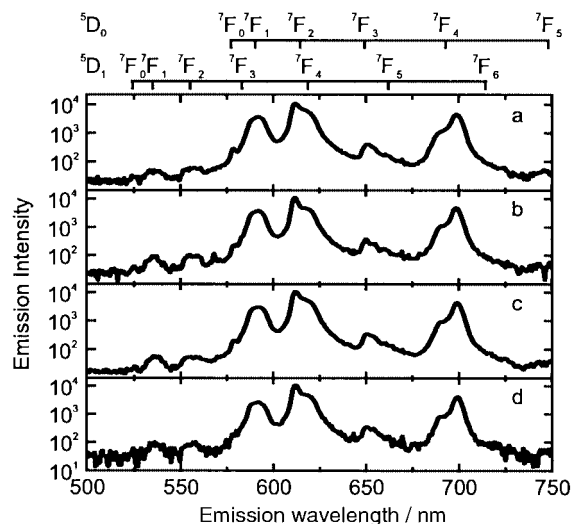
Fig. 5 Emission spectra from the 5 D 1 and 5 D 0 states of the EuH n (pmdp) l complexes present in the solutions of Table 4 normalized to the same intensity for the peak at 611.8 nm. Total concentrations of pmdp were (a) 0.00746 M, (b) 0.01127 M, (c) 0.01893 M and (d) 0.02922 M. The assignments of the observed bands appear above along with tick marks denoting the expected centers 40 of aquated Eu 3+ emission bands.
